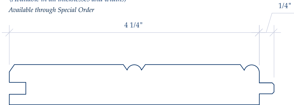
IL 916 Shown as 11/16 x 4 1/2 (Available in all thicknesses and widths) Available through Special Order
