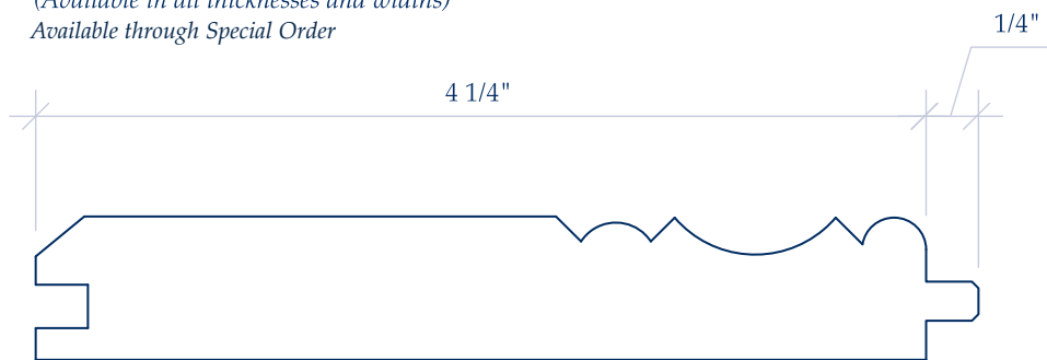
IL 917 Shown as 11/16 x 4 1/2 (Available in all thickness and widths) Available through Special Order
