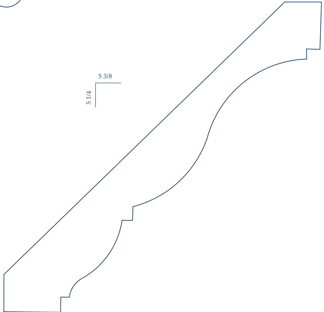
IL E03 Available through Special Order 1 1/8 x 7 1/2
