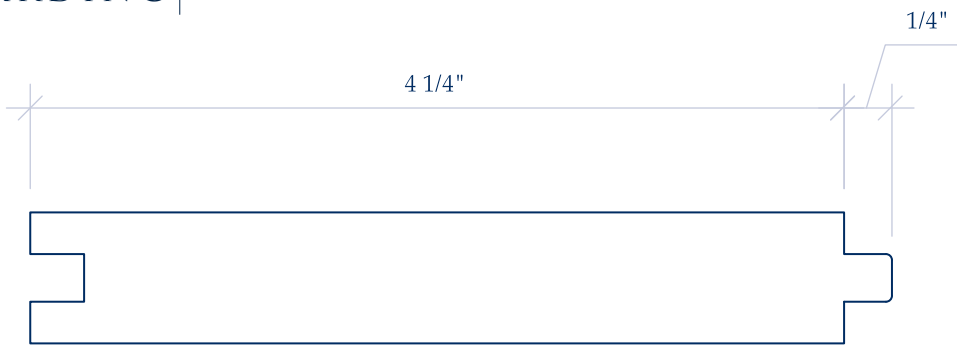
IL 910 Shown as 11/16 x 4 1/2 (Available in all thicknesses and widths) Available through Special Order
