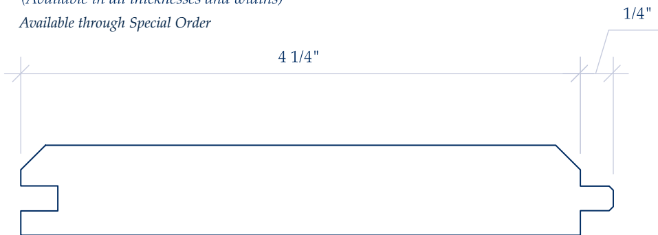
IL 915 Shown as 11/16 x 4 1/2 (Available in all thicknesses and widths) Available through Special Order
