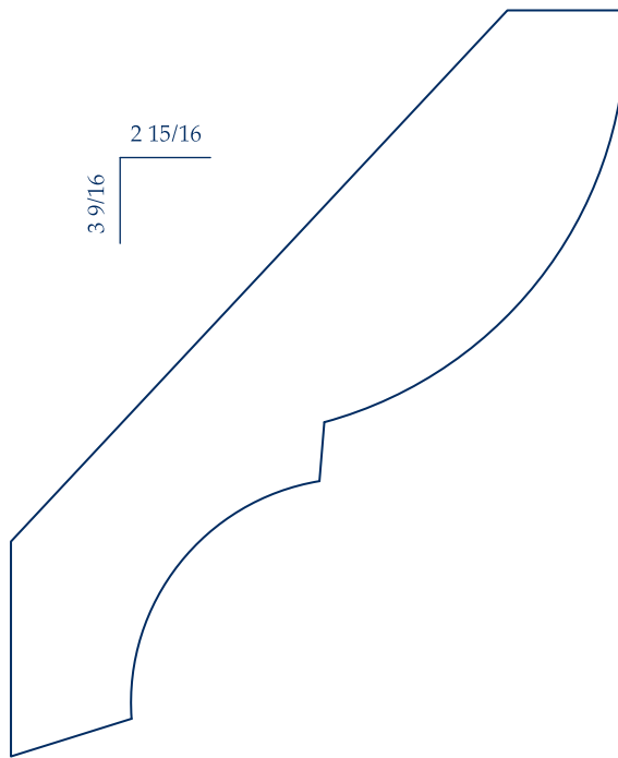
IL E07 Available through Special Order 1 x 4 5/8
