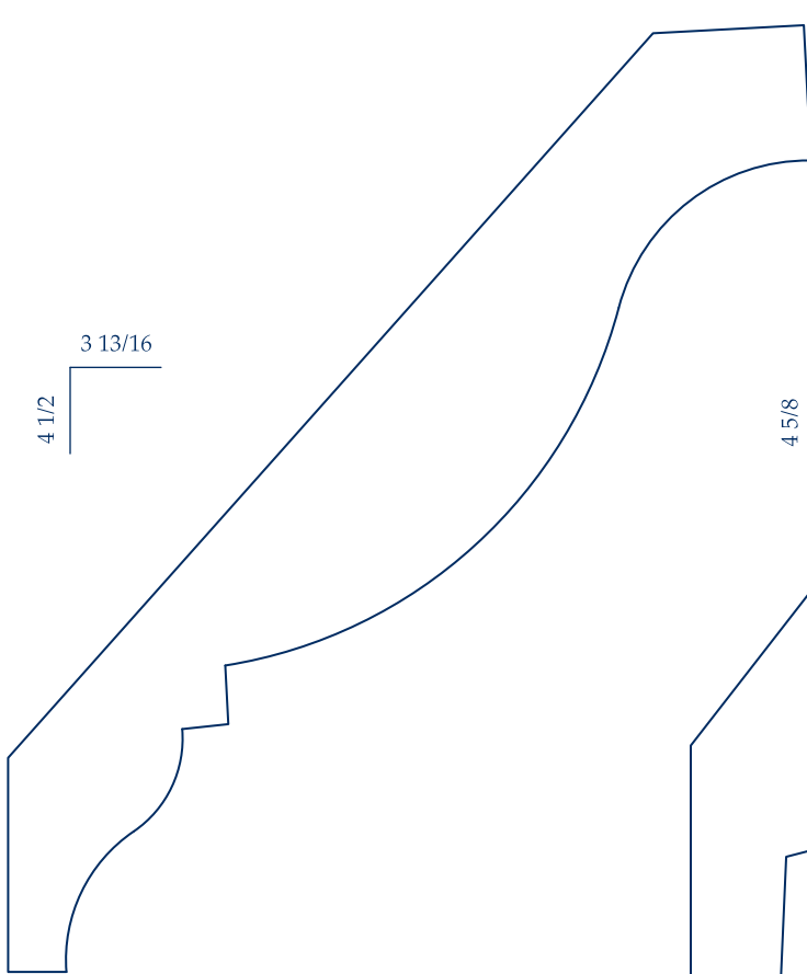
IL E04 Available through 1 x 5 7/8 Special Order
